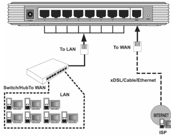
Figure 3-1 Hardware Installation of the TL-R860 Cable/DSL Router
